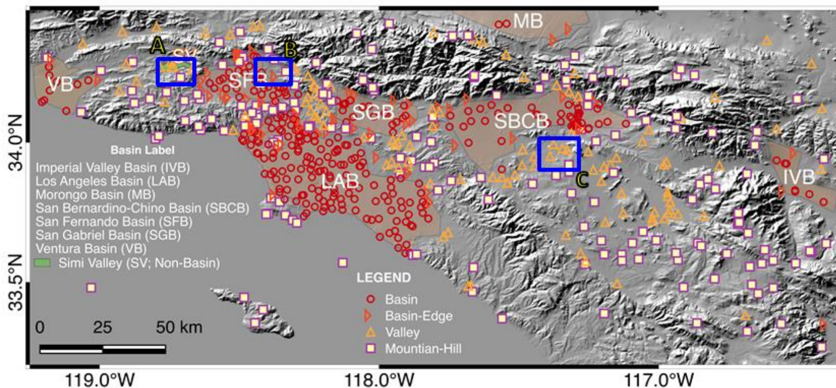
Figure 4. Detail map of southern California showing ground motion stations and sedimentary basins and related features considered in this paper. Ground motion sites are plotted according to a morphology-based site categorization scheme proposed in this paper. Boxes A, B, and C are detailed in subsequent figures in this paper.
