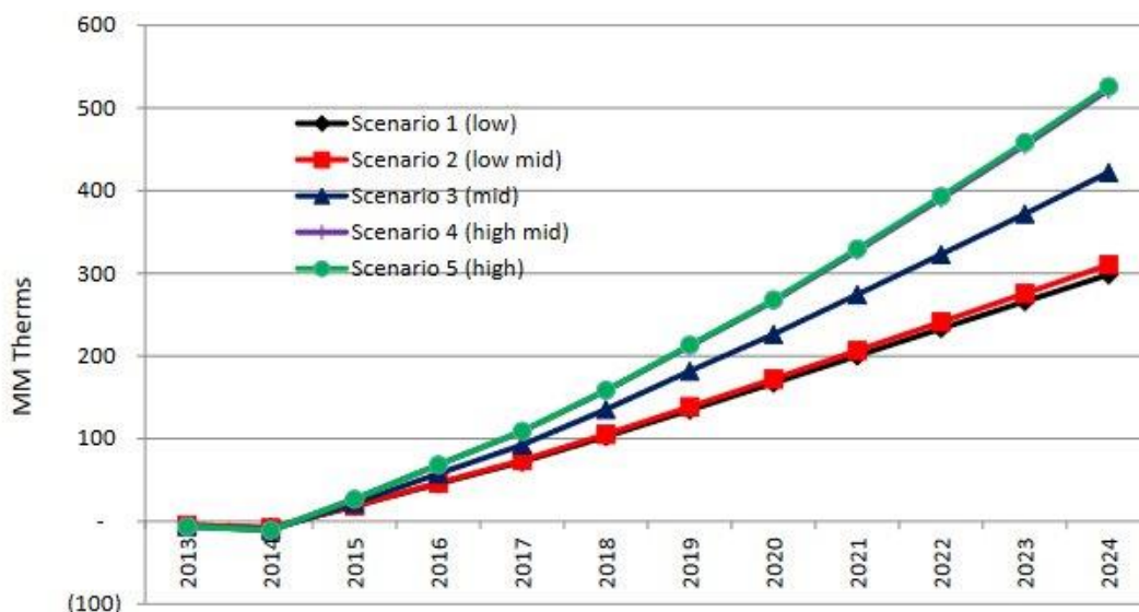
Figure 24. Adopted Natural Gas AAEE.
