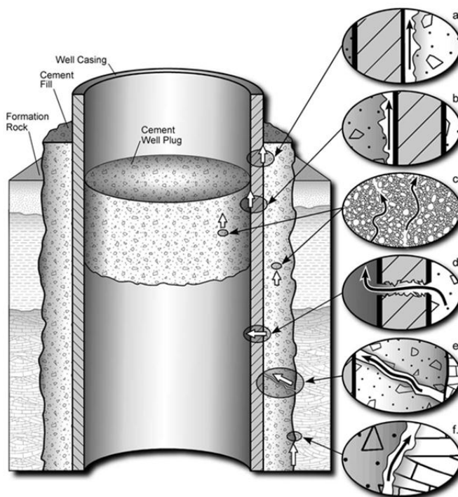
Figure 1.2-3. Three-dimensional cross section of a generic well (in this case shown with a cement plug for discussion purposes) showing production casing, cement, and formation along with various failure modes (a) bad seal between casing and cement; (b) bad seal between cement plug and casing; (c) leakage through the cement pore space as a result of cement degradation; (d) leakage through casing as a result of corrosion; (e) leakage through fractures in cement; and (f) leakage between cement and rock. From Gasda et al. (2004) (drawing by Dan Magee, Alberta Geol. Survey).
