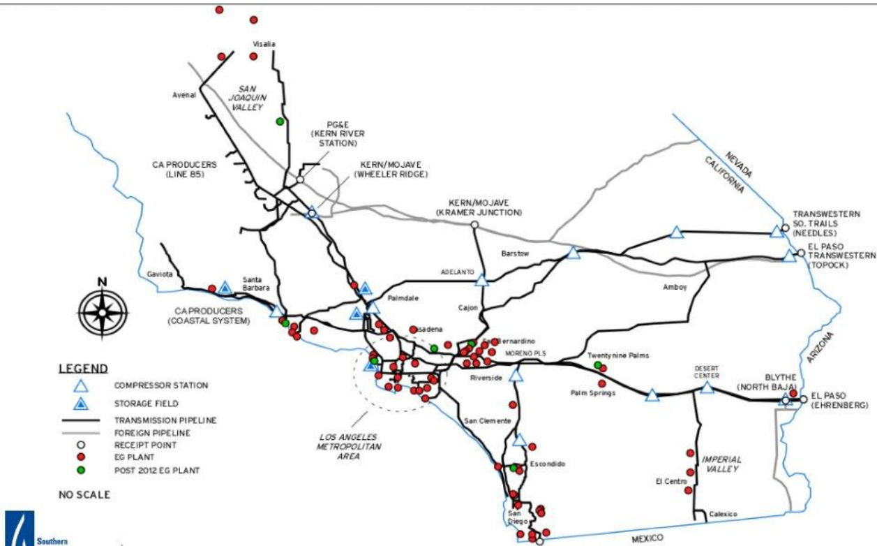
Figure 20. SoCalGas and SDG&E Electricity Generation Customer Locations Source: SoCalGas DOE QER Presentation
