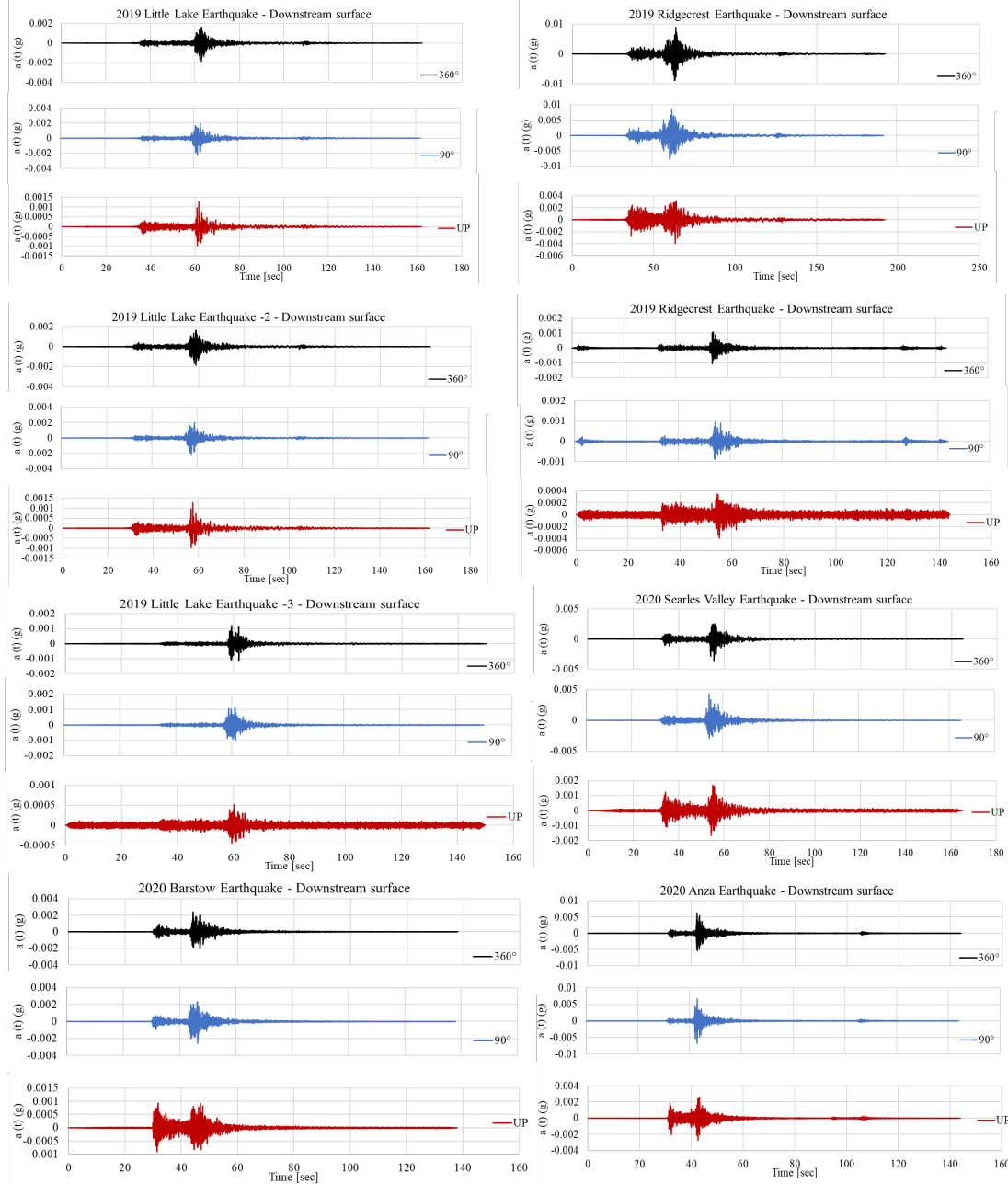
Figure 7. Acceleration time histories recorded downstream site (cont'd)
