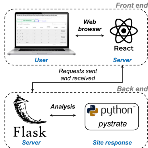
Figure 3. Web application tool architecture and request response-cycle. Generate Ground Motions for Nonlinear Deformation Analyses
