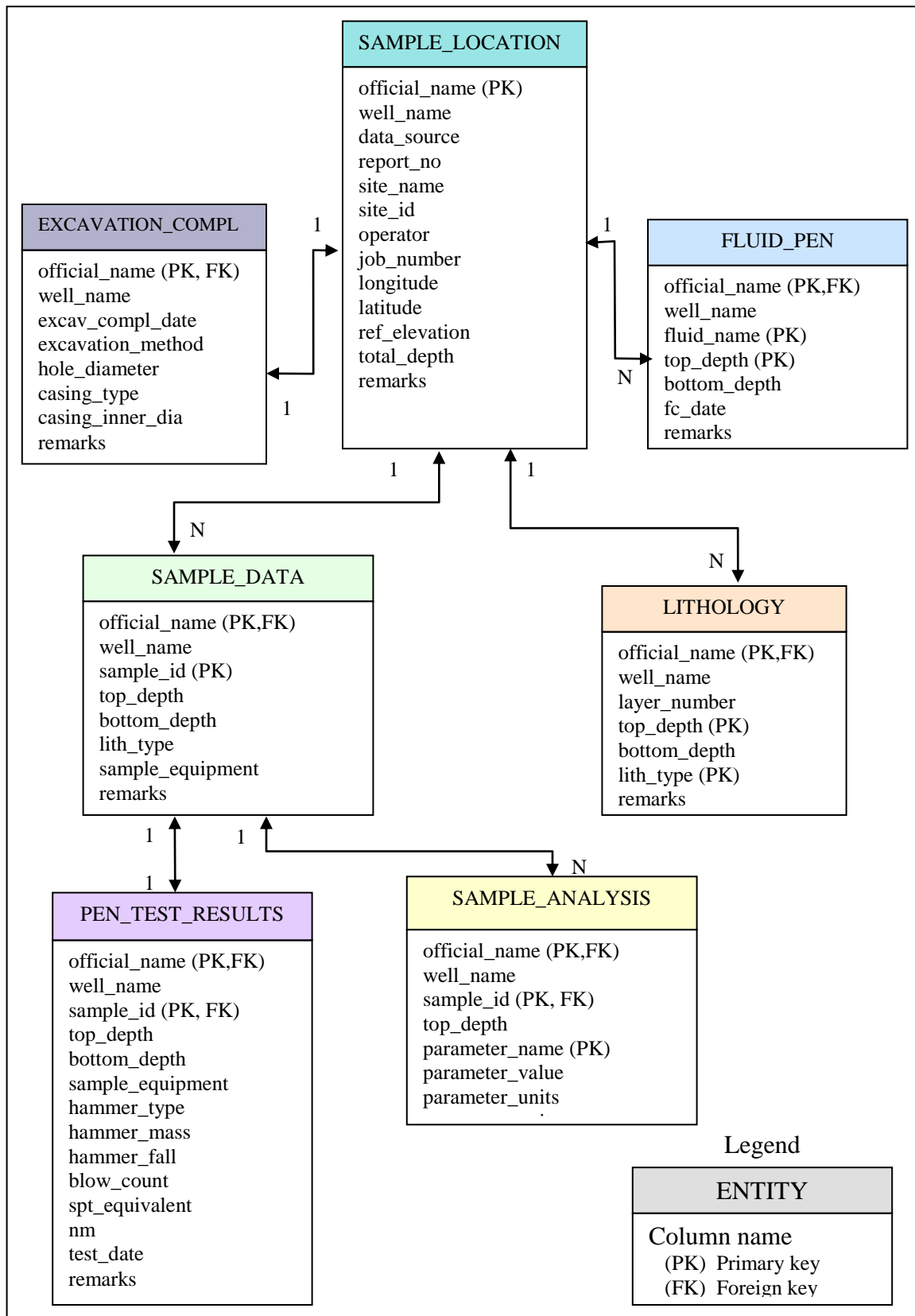
Entity Relationships Diagram — Web Data Model
