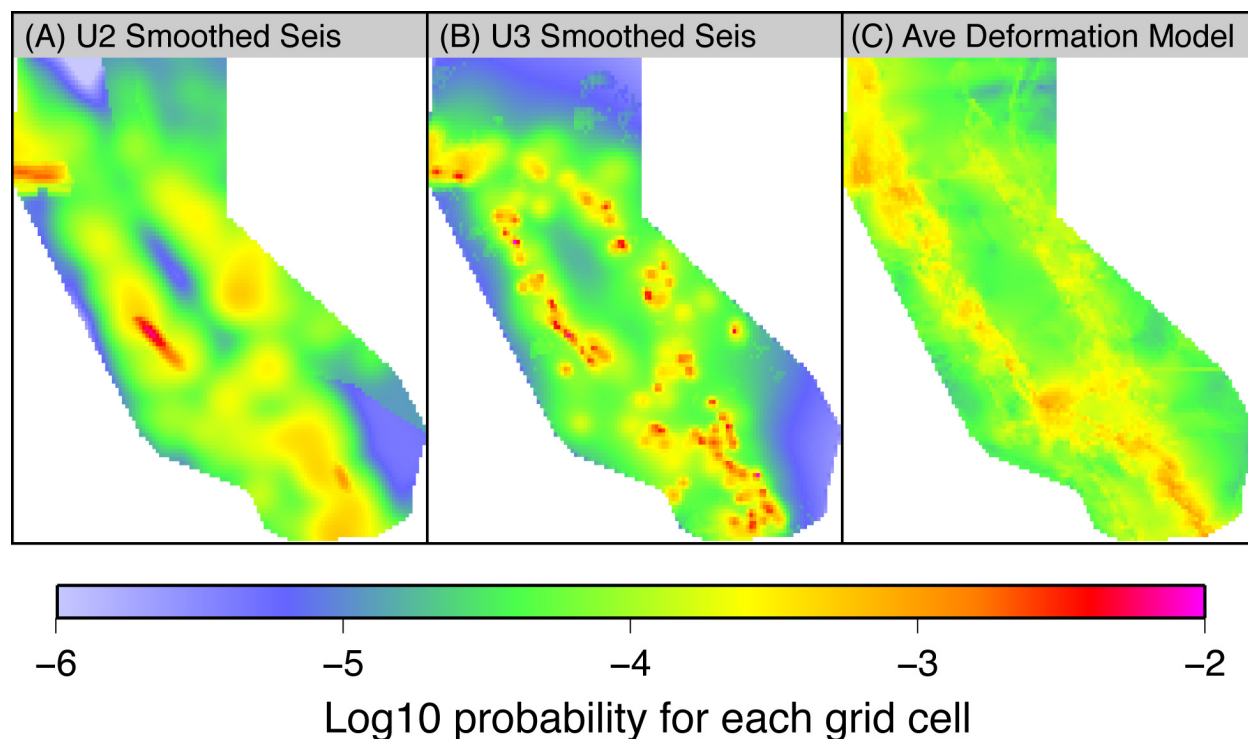
Figure 14. Maps showing the various off-fault spatial seismicity probability density functions (SpatialPDF) used in UCERF3 for setting gridded seismicity (referred to as the Off-Fault Spatial Seis PDF logic tree branch in figure 3). Values in each map sum to unity. A , The UCERF2 Smoothed Seismicity model. B , The UCERF3 Smoothed Seismicity model of Felzer (appendix M, this report), which has a higher resolution, adaptive smoothing kernel. C , SpatialPDF implied by the average of the off-fault moment rate maps from appendix C (this report), which includes the Average Block Model, NeoKinema, and Zeng deformation models, and averages over maps for both Fault Models 3.1 and 3.2.
