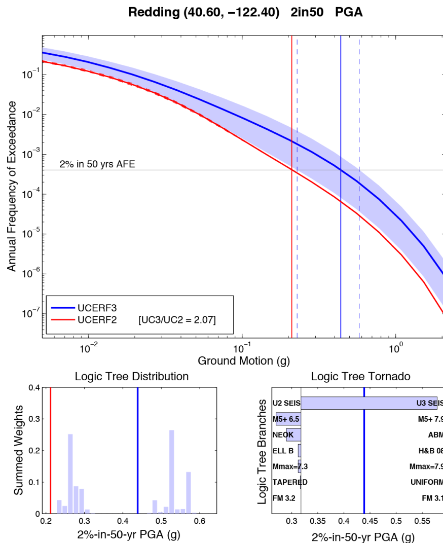
Figure 30. Graphs illustrating the hazard-curve example for PGA at the Redding site listed in table 13 .
